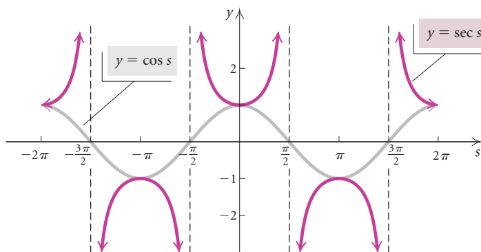
The secant function
