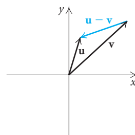
\mathbf{u} - \mathbf{v} is the vector from the terminal point of \mathbf{v} to the terminal point of \mathbf{u} .
