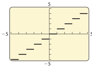
y = \text{int}(x) , DOT mode
