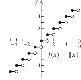
Greatest integer function
