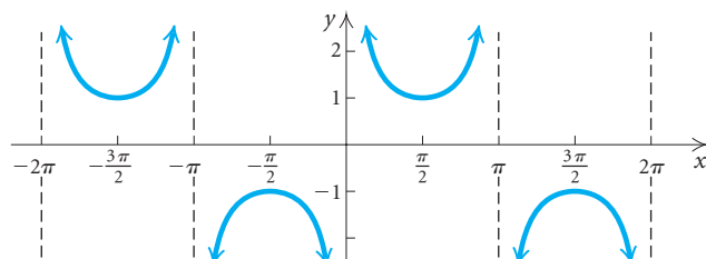
The cosecant function: f(x) = \csc x
