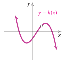
A discontinuous function
